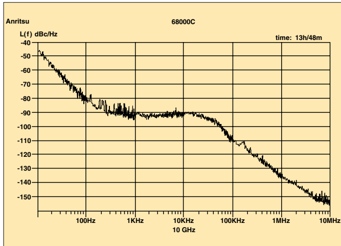
Typical 68C single-sideband phase noise at 10 GHz carrier.
